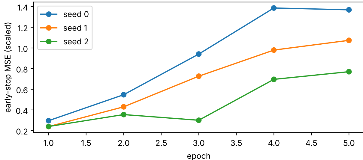
Early stopping
